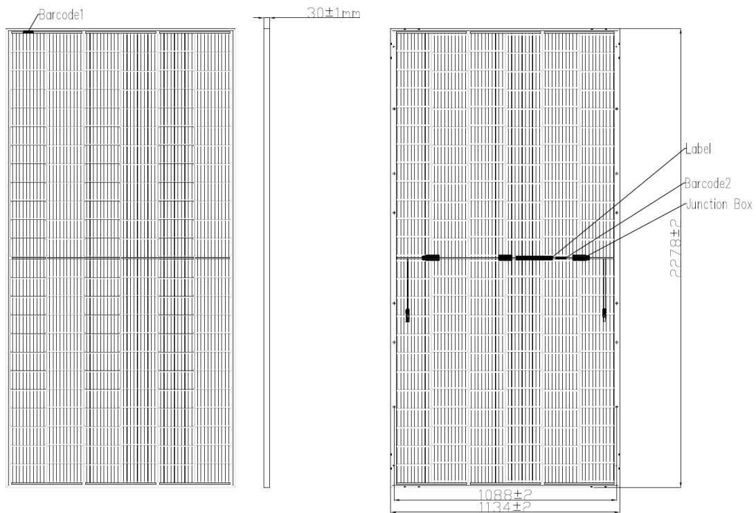
144 Cell bifacial double glass Module
